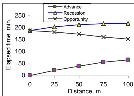
Fig. 5: Advance-Recession-Opportunity curves for perforated tubes system under 100m ridge(double furrow) length (L100) slope 0.1%.
