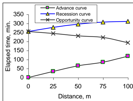
Fig. 2: Advance-Recession-Opportunity curves for traditional irrigation method under 100 m border length (L100).
