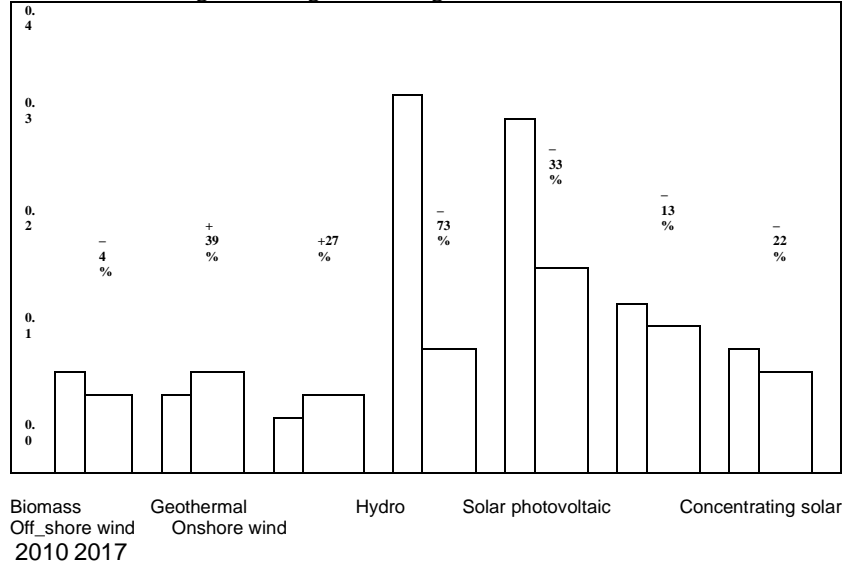
Shape (2-1) : Global levelized cost of electricity from utility-scale renewable power-generation technologies, 2010/2011 – 2017/2018 2016 US$/KwH, global weighted average
