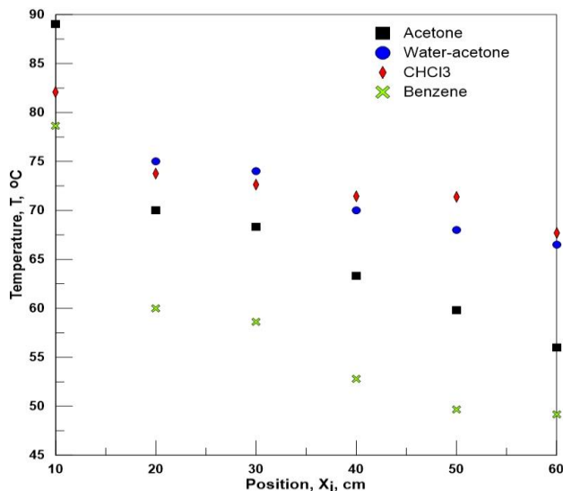
Figure. 4. Average temperature distribution along 25% filled thermosyphon for different working fluids at 1400 rpm.
