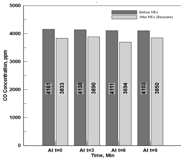
Figure. 15. Carbon monoxide concentration before and after attaching the heat exchanger at 1400 rpm, FR=50% benzene.
