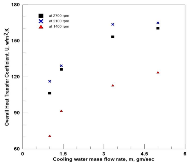
Figure. 9. Overall heat transfer coefficient at different cooling rates for FR=25% benzene at different engine speeds.
