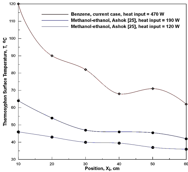
Figure. 14. Temperature distribution comparison between this case study and Ashok’s experiment
