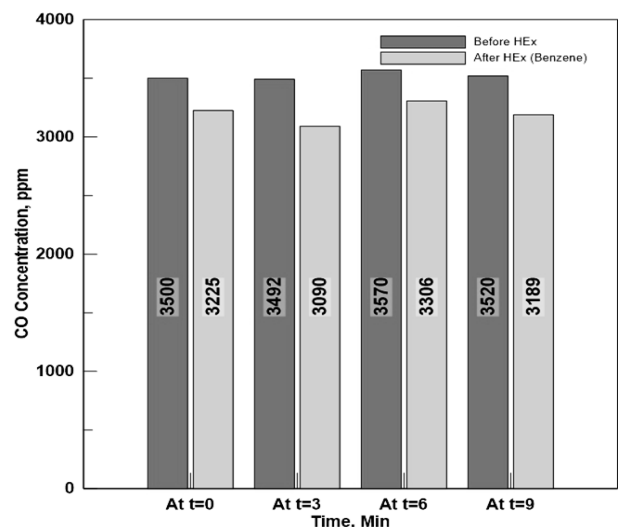
Figure. 16. Carbon monoxide concentration before and after attaching the heat exchanger at 2100 rpm, FR=50% benzene.
