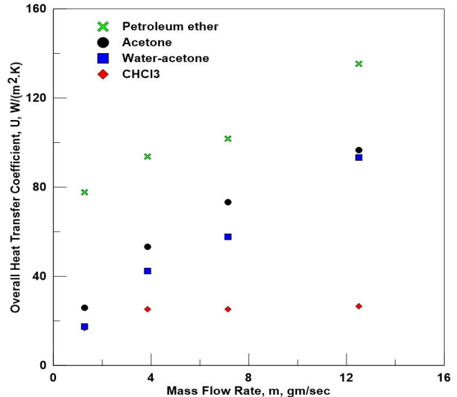
Figure. 5. Overall heat transfer coefficient at different cooling rates for FR=25% different working fluids at 1400rpm.
