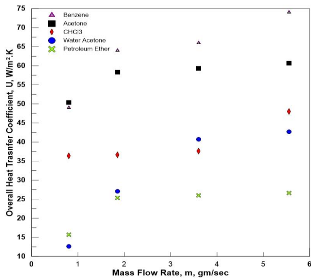
Figure. 7. Overall heat transfer coefficient at different cooling rates for FR=50% different working fluids at 1400rpm
