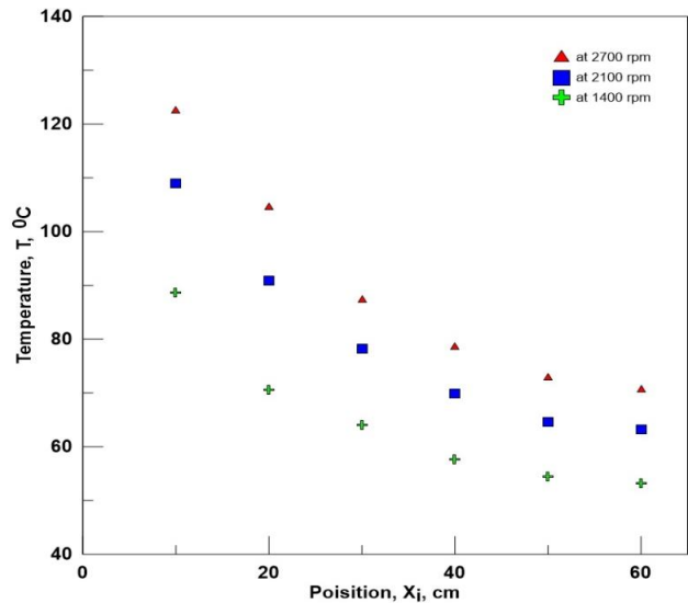
Figure. 8. Average temperature distribution along FR=25% benzene filled thermosyphon for at different engine speeds.
