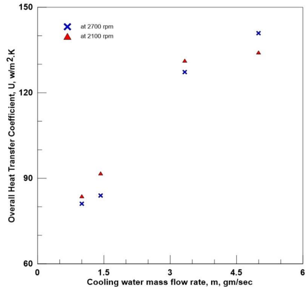
Figure. 13. Overall heat transfer coefficient at different cooling rates for FR=100% benzene at different engine speeds.
