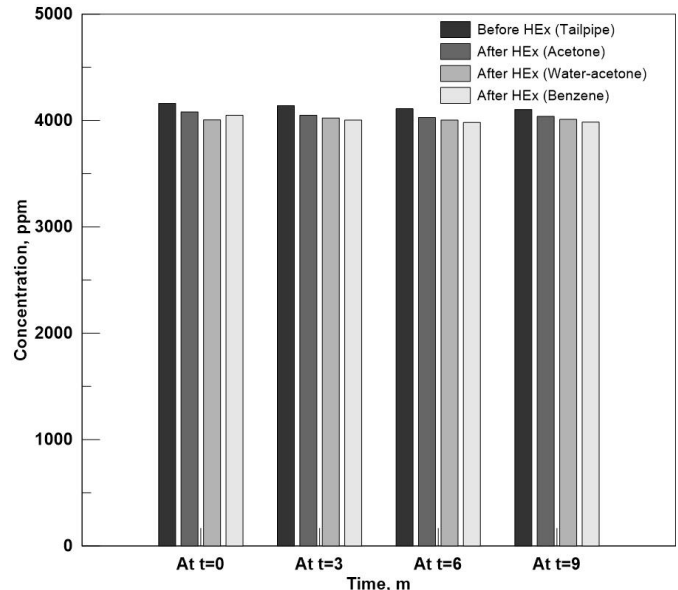
Figure. 6. Carbon monoxide concentration comparison at tailpipe and after heat exchanger charged with FR=25% of various working fluids at 1400 rpm
