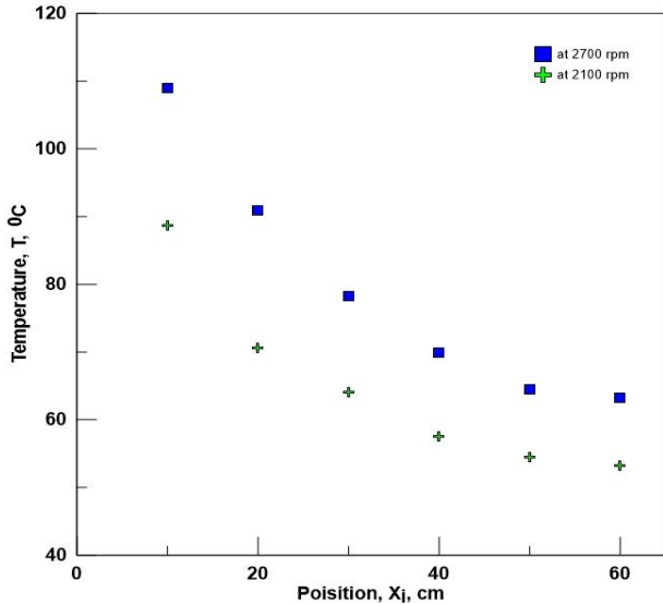
Figure. 10. Average temperature distribution along FR=50% benzene filled thermosyphon for at different engine speeds.
