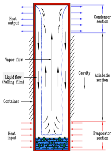
Figure 1. Thermosyphon sections and working principle
