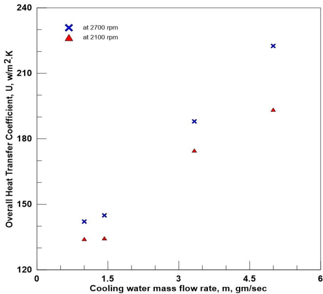
Figure. 11. Overall heat transfer coefficient at different cooling rates for FR=50% benzene at different engine speeds.
