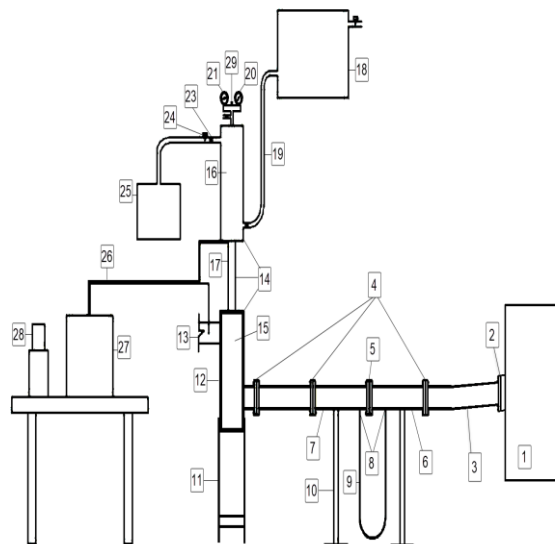
Figure 2. Experiment test rig layout
