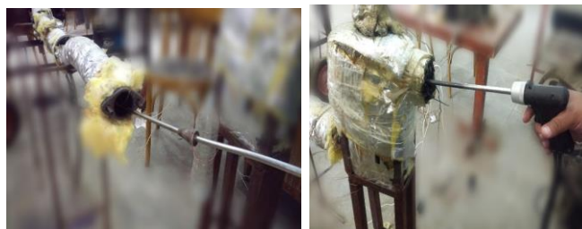
Figure 3(a). Probe intakes sample-before heat exchanger Figure 3 (b) Probe intakes sample after heat exchanger.
