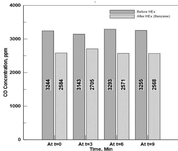
Figure. 17. Carbon monoxide concentration before and after attaching the heat exchanger at 2700 rpm, FR=50% benzene.
